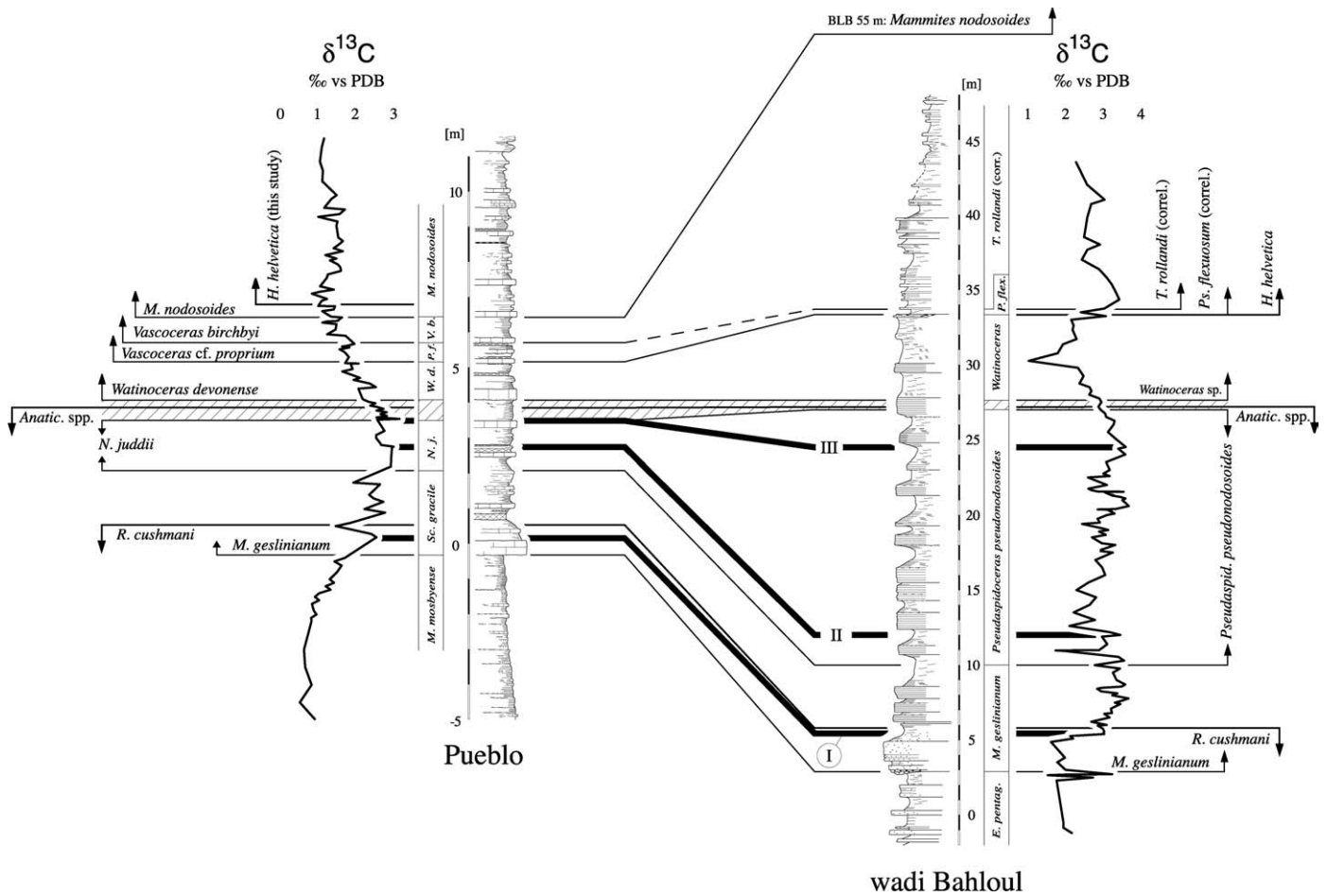
Fig. 11. Long-distance correlation of reference-levels: biostratigraphic (FO & LO of ammonite and planktic foraminifera marker species) and geochemical datum lines ( \delta^{13}C peaks) from the Pueblo section (Colorado) to the wadi Bahloul section (Central Tunisia).
