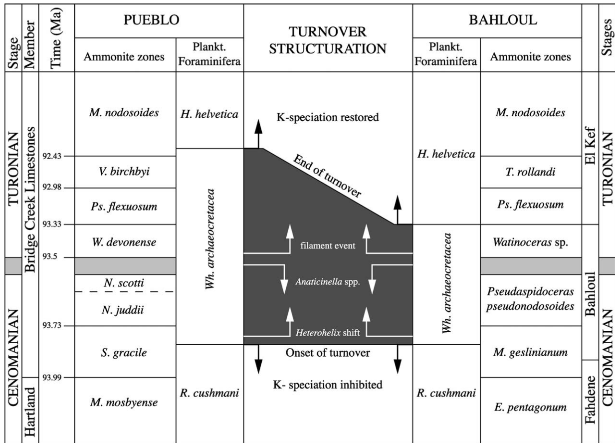
Fig. 13. Planktic foraminiferal turnover during the Cenomanian–Turonian boundary interval at Pueblo and wadi Bahloul. Structure and diachroneity of this turnover relative to the chronostratigraphy and the ammonite zonation. Note position of the three bio-events that structure this interval: Heterohelix shift, LO of Anaticinella sp. and “filament” event. The light gray shadow marks the precision interval; dark gray shadow marks the lengths of dominance time of r -speciation that correspond to the diachronism of the Whiteinella archaeoretacea Zone from Pueblo to Bahloul area.
