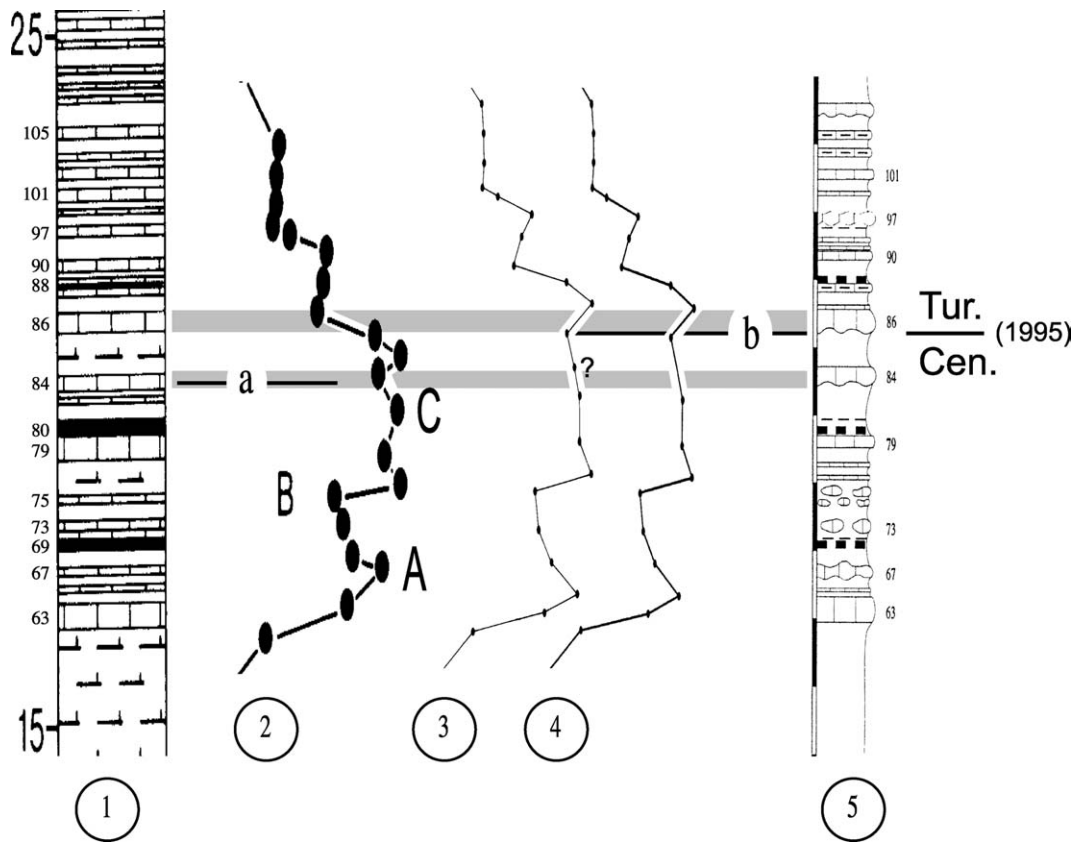
Fig. 12. Comparison of \delta^{13}\text{C} curves published for the Pueblo section. 1, lithologic profile of the borehole, PU-79-Pueblo core in Pratt (1982), Pratt (1984) and Pratt and Threlkeld (1984). 2, \delta^{13}\text{C}_{\text{org}} curve of Pratt and Threlkeld (1984), and Pratt (1985), with details of the positive excursion: A = first peak; B = a brief decrease; C = plateau of values before the descending phase. 3, \delta^{13}\text{C}_{\text{org}} curve of Pratt and Threlkeld (1984) reproduced in Gale et al. (1993) referred to as “original from Pratt and Threlkeld (1984) and from Pratt et al. (1993)”. Note the additional point marked here (?) that causes a stretching of the original curve. 4, \delta^{13}\text{C}_{\text{org}} curve reproduced in Kennedy et al. (2000: Fig. 9). Note that the additional point has been removed whereas the stretching remains. 5, lithologic profile of the Pueblo section, published by Cobban (1985), and by Kennedy and Cobban (1991). Dark horizontal lines : a = early position of the C/T boundary in bed 84 according Cobban and Scott (1972), as published in Pratt (1982, 1984, 1985) and Pratt and Threlkeld (1984); and b = position of the C/T boundary at the base of bed 86 as defined by Kennedy and Cobban (1991). Thick light grey bands underline lithologic correlation of beds 84 and 86.
