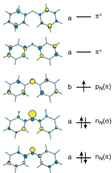
Figure 2. MOs of 2 involved in the electronic transitions of 2^+ , 2^+ , and 2^- (electronic ground configuration for 2^+ is shown). Note that some occupied \pi MOs lie between the two n_{\text{N}} MOs.
