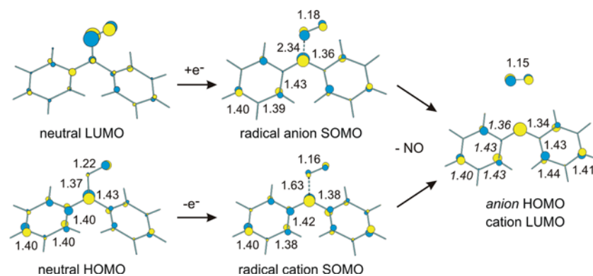
Figure 8. Change in bond lengths and frontier MOs on ionization of 1 and subsequent loss of NO* from the resulting radical ions, 1 •+ and 1 •- (SOMO = singly occupied MO), to yield the closed-shell ions, 2 + and 2 - , respectively, as calculated by the B3LYP/6-31G* method (see Supporting Information for full geometries).
