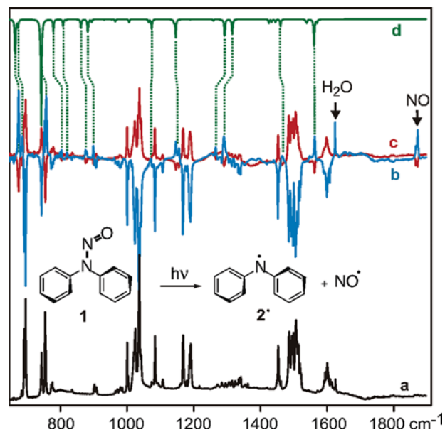
Figure 3. Changes in the IR spectra upon photodissociation of 1 (b) and its re-formation by NIR irradiation (c) in an Ar matrix. (a) Absolute spectrum of 1 . Top: IR spectrum of 2^+ calculated by B3LYP/6-31G*.
