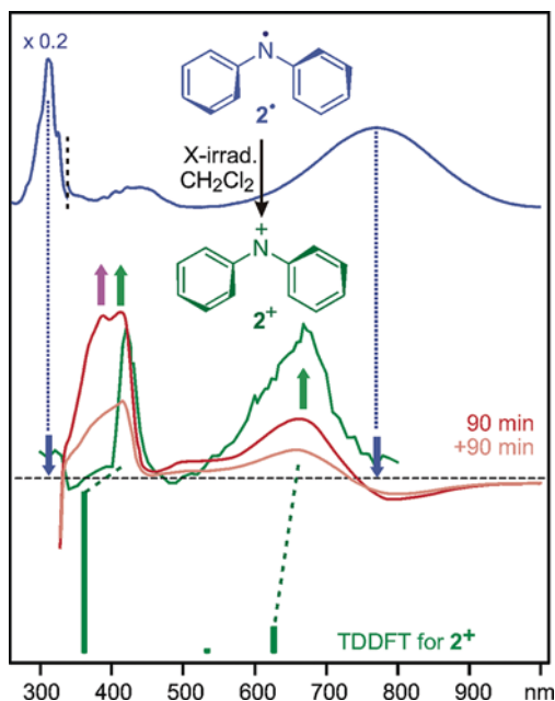
Figure 4. Spectral changes on X-irradiation of a \text{CH}_2\text{Cl}_2 -doped Ar matrix containing aminyl radical 2^{\bullet} (blue spectrum) for 90 min (red spectrum) and then another 90 min (orange spectrum). The green trace is a copy of the spectrum of 2^+ obtained by Moran and Falvey by flash photolysis of the N -diphenylaminopyridinium tetrafluoroborate in \text{CH}_3\text{CN}/\text{CF}_3\text{COOH} . 29 Bottom: TD-B3LYP predictions of the electronic transitions of 2^+ (for details, see Supporting Information).
