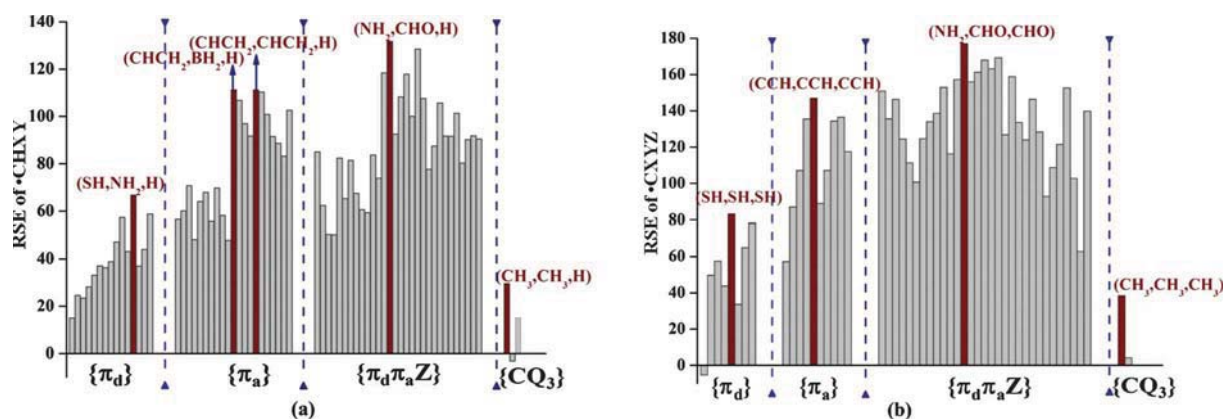
Fig. 2 Calculated radical stabilization energies (RSEs in kJ mol -1 ) for (a) disubstituted radicals ( \cdot CHXY ) and (b) trisubstituted radicals ( \cdot CXYZ ) in the \{\pi_d\} , \{\pi_a\} , \{\pi_d\pi_aZ\} and \{CQ_3\} sets.
