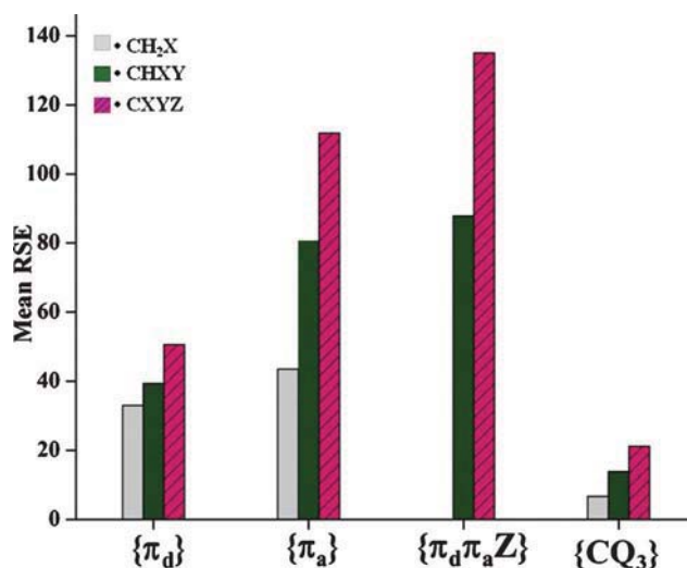
Fig. 4 Comparison of mean RSEs in \text{kJ mol}^{-1} for mono-, di-, and tri-substituted radicals for the \{\pi_d\} , \{\pi_a\} , \{\pi_d\pi_aZ\} and \{\text{CQ}_3\} sets.
