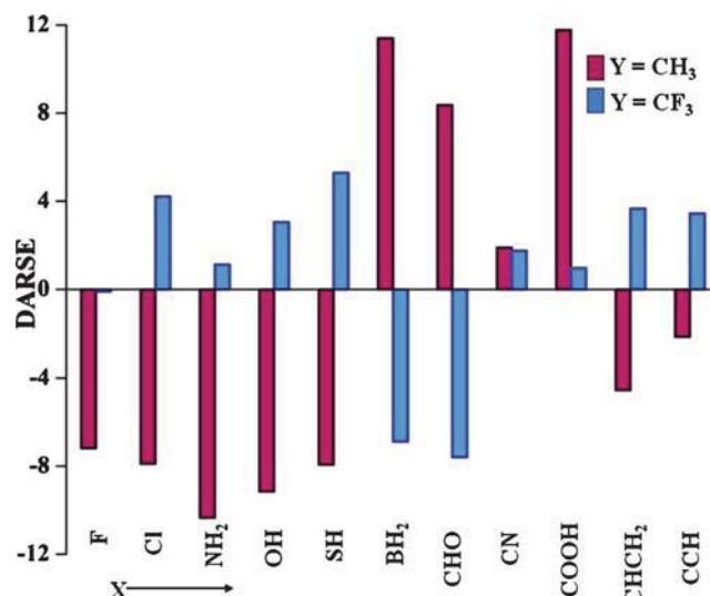
Fig. 12 Deviations from additivity of RSEs (DARSEs, \text{kJ mol}^{-1} ) for \cdot\text{CHXY} radicals in the \{X-CQ_3\} set with Y = \text{CH}_3 and \text{CF}_3 .
