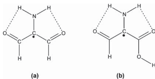
Fig. 21 Hydrogen-bonding interactions in the (\text{NH}_2, \text{CHO}, \text{CHO}) and (\text{NH}_2, \text{CHO}, \text{COOH}) radicals.
