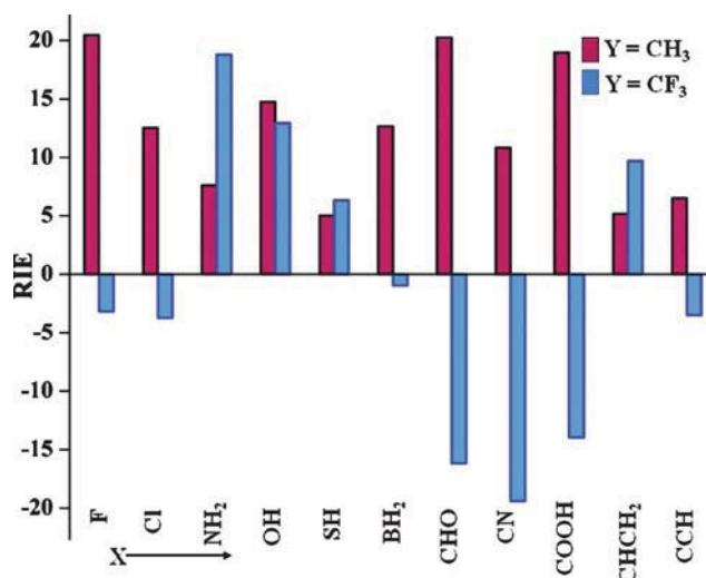
Fig. 7 Radical interaction energies (RIEs, \text{kJ mol}^{-1} ) for \cdot\text{CHXY} radicals in the \{\text{X-CQ}_3\} set for Y = \text{CH}_3 and \text{CF}_3 .
