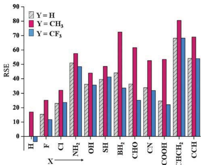
Fig. 3 Comparison of RSEs ( \text{kJ mol}^{-1} ) for \cdot\text{CHXY} radicals in the \{\text{X-CQ}_3\} set, with \text{Y} = \text{H} , \text{CH}_3 or \text{CF}_3 .
