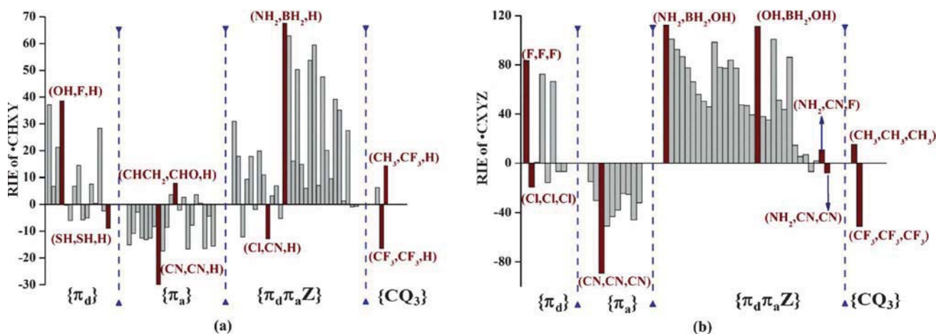
Fig. 5 Calculated radical interaction energies (RIEs, \text{kJ mol}^{-1} ) for (a) disubstituted radicals ( \cdot\text{CHXY} ) and (b) trisubstituted radicals ( \cdot\text{CXYZ} ) in the \{\pi_d\} , \{\pi_a\} , \{\pi_d\pi_aZ\} and \{\text{CQ}_3\} sets.
