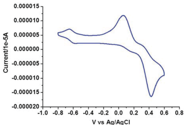
Fig. 6 Cyclic voltammogram of complex 3.
