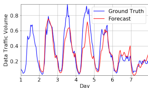
(a) MuLSTM forecast
