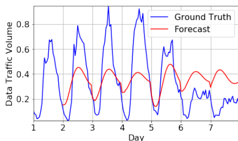
(b) ARIMA forecast
