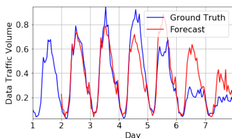
(c) WANN forecast
