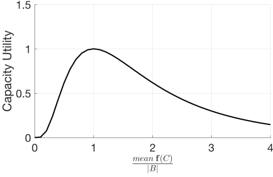
Figure 4. The curve of the designed capacity utility function, which reaches its maximal when the cluster traffic volume equals the BBU capacity.
