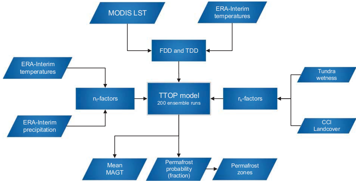
Fig. 1. Flowchart of the employed methodology. The TTOP model was run 200 times with varying n_f -factors and r_k -factors according to subpixel statistics.
