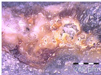
Figure 61 : 1004-22, MO, DF, 50x ©HECR-Arc, 2013.
