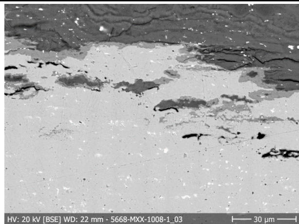
Fig. 7: SEM image of the metal sample a, from Fig. 6 (detail), BSD-mode.
