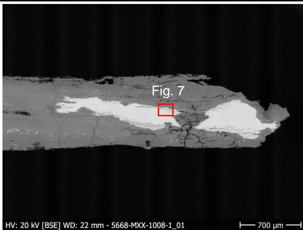
Fig. 6: SEM image of the metal sample a, from Fig. 4, BSD-mode.
