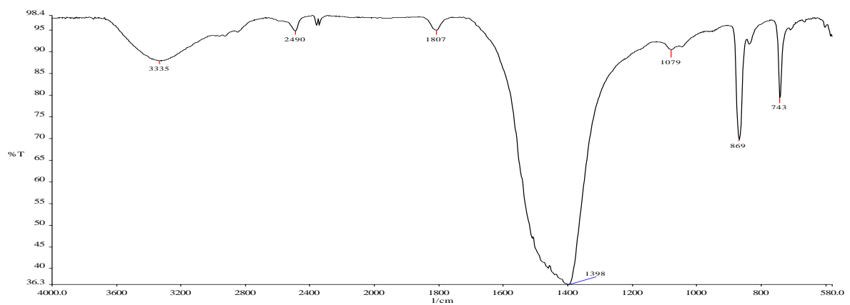
Figure 144 : Spectre FTIR (transmission), 1008-1a, particule noire CS : smithsonite [1395, 869, 743 cm -1 ] © HKB, 2013.
