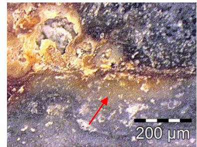
Figure 87 : Interface CP1e/CM1(B), 1004-22, MO, DF, 50x ©HECR-Arc, 2013.
