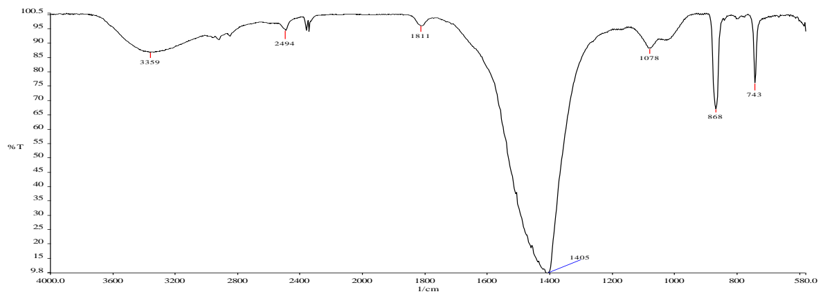
Figure 143 : Spectre FTIR (transmission), 1008-1a, particule blanche : smithsonite [1405, 868, 743 cm -1 ] © HKB, 2013.
