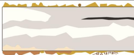
Fig. 3: Schematic interpretation of the cross-section of the object. We can see elements from soil at the surface, and corrosion products of different colours occurring as layers.
