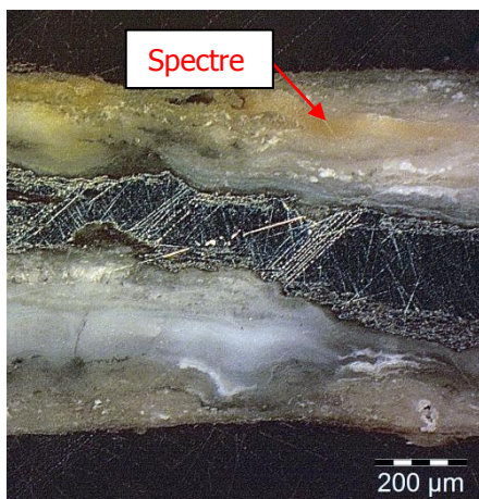
Figure 70 : Localisation du spectre EDS, 1008-1a, MO, DF, 50x ©HECR-Arc, 2013.
