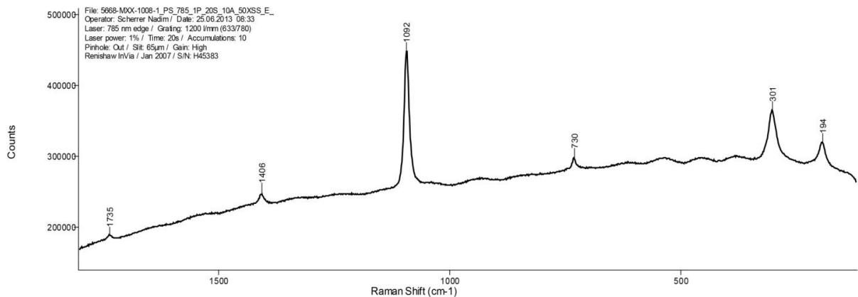
Figure 147 : Spectre Raman, 1008-1a, zone noire : smithsonite (ZnCO 3 ) [1735, 1407, 1093vs, 731, 302s, 194m cm -1 ] ©HKB, 2013.
