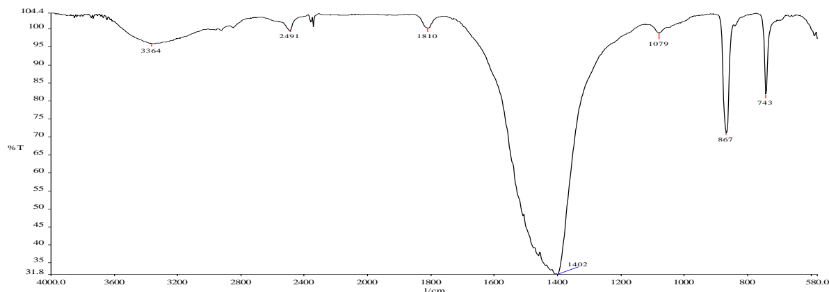
Figure 67 : Spectre FTIR (transmission), 1008-1a, particule grise : smithsonite [ 1402, 867, 743 \text{ cm}^{-1} ] ©HKB, 2013.
