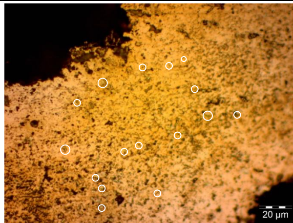
Fig. 8: Micrograph of the metal sample b, etched, bright field, 500x.
