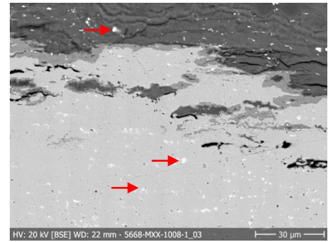
Figure 48 : Inclusions de plomb, image SEM, BSE, 1008-1a, ©IMA, 2013.
