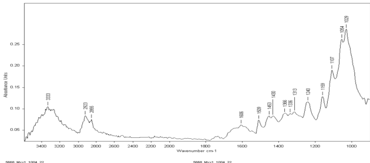
Figure 55 : Spectre FTIR de la cellulose (ATR FPA Imaging), 1004-22 ©HKB, 2013.
