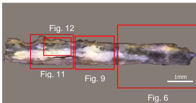
Fig. 4: Micrograph of the cross-section (sample a) showing the locations of next figures. Unetched, dark field, 50x.
