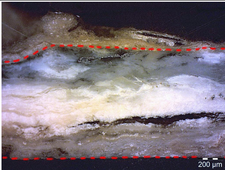
Fig. 11: Micrograph of the metal sample a, from Fig. 2 unetched, dark field, 50x. View of the inner layers and the limit of the original surface (red line). We can see that the interfaces between the different layers are not well defined: some of the white corrosion product is found inside the inner grey layer.
